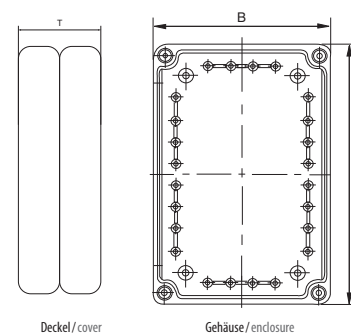
Deckel / cover
